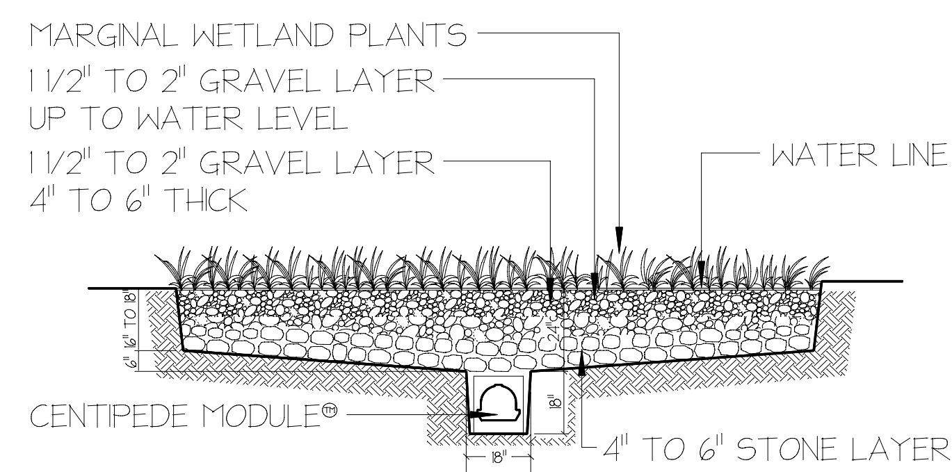
WETLAND DETAIL © AQUASCAPE DESIGNS 2005
